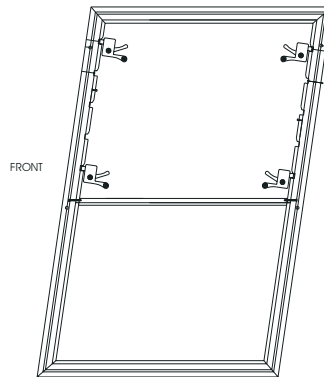
OUTSIDE VIEW LEFT HAND SHOWN RIGHT HAND SYM OPP
