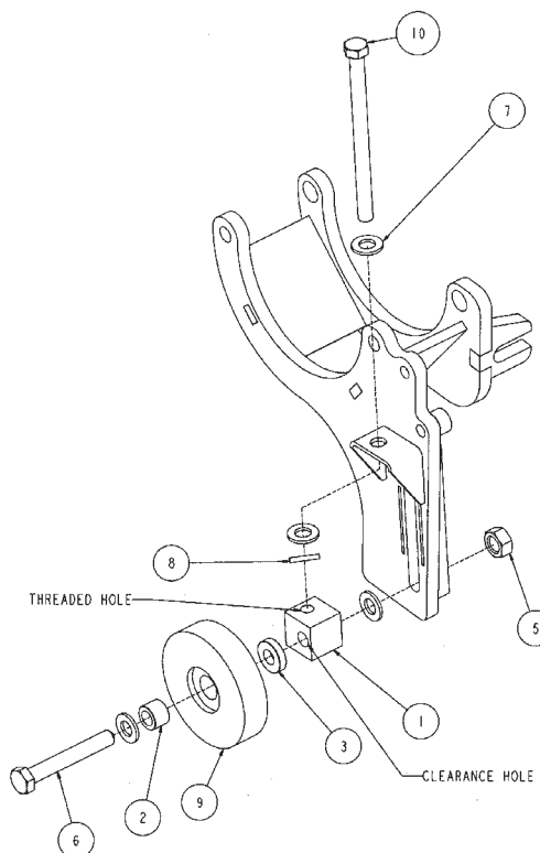
Compressor Mount Kit 184251 Assembly 184253
